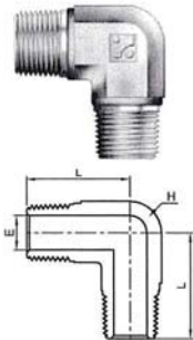
Male NPT Threads
