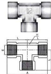
Female NPT Threads
